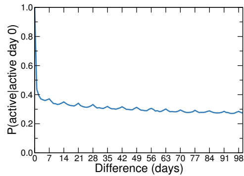
Figure 1: Auto-correlation of download activity reveals weekly periodicities and high probability of activity on the following day.
