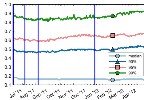
(b) Probability of staying active ( p_1 )
