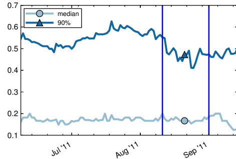
(b) Probability of staying active ( p_1 )
