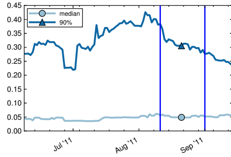
(a) Probability of becoming active ( p_{00} )
