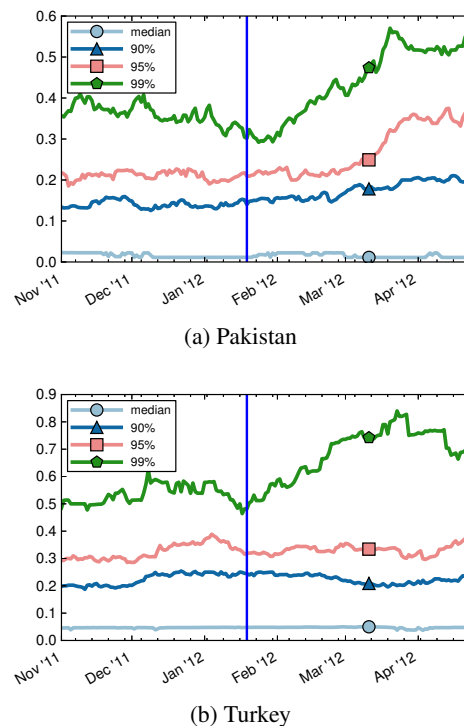
Figure 4: Growing activity ( p_{00} ) following the shutdown of MegaUpload on January 19, 2012 (vertical line). The “median” curve captures activity levels of typical users; the other 3 curves show the same for increasingly heavy users.
