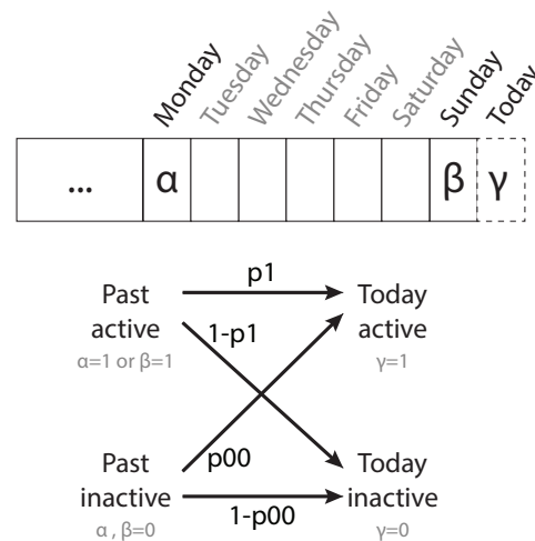
Figure 2: Diagram of hidden Markov model input variables (top) and parameter and state transitions (bottom).
