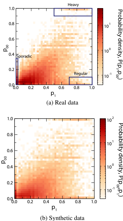
Figure 3: Joint probability distribution of p_{00} and p_1 parameters for entire sample population (a), and with synthetic data generated from model parameters (b). We identify clusters of users in the real data.
